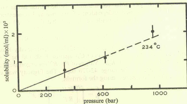
FIG. 7.—Solubility isotherm for the system Ar + AgNO_3 .
